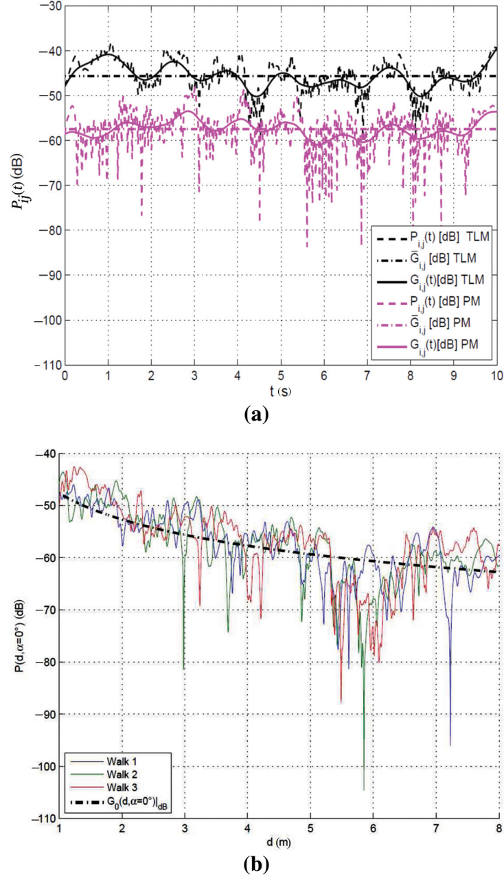
Figure 5.14 Channel gains for different movements [RVD14, RDV12] (a) Walking side by side, and (b) One subject walking towards the other.
