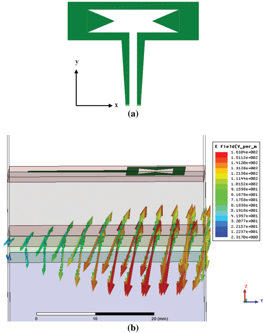
Figure 5.3 Creeping wave ANT and its vector electric field [GHP + 12, YY11a] ©2011.
