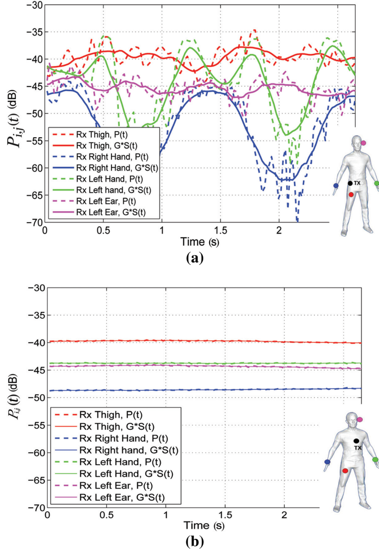
Figure 5.8 On-body channel power transfer functions in indoor: (a) Walking, and (b) Still.
