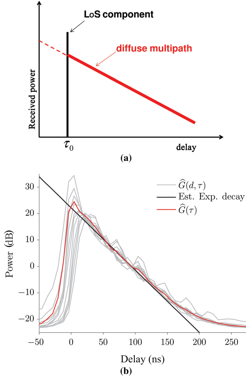
Figure 3.1 (a) Power delay profile (PDP) modelling according to the room electromagnetics (REM) theory, (b) spatially averaged PDPs obtained for transmitter-receiver distance intervals of 4\lambda for receiver positions [SPF+ 12, SPF+ 13b].
