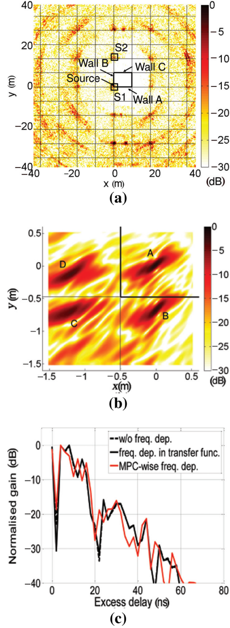
Figure 3.6 (a) Overall map of image source distribution and (b) enlarged map for the source group S1; and (c) effect of the multipath component (MPC)-wise frequency dependence [HRM12].
