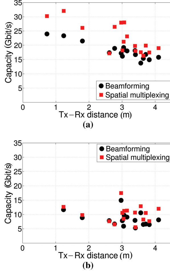
Figure 3.15 Comparison of the ergodic channel capacity for beamforming and spatial multiplexing. (a) 9 \lambda^2 antenna aperture size, and (b) NLoS scenario with antenna aperture size of 9 \lambda^2 [HGW13].
