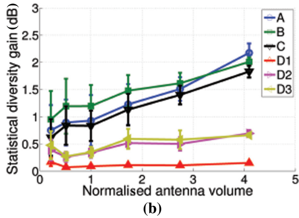
Figure 3.5 Dependence of the attainable spatial diversity gain against the volume of a cubical hollow array at 6 GHz, in an industrial room scenario [HTKD11].
