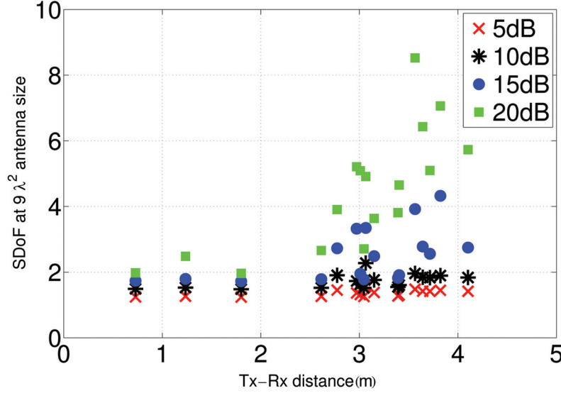
Figure 3.14 Distance dependency of the spatial degrees-of-freedom (SDoF) for an antenna aperture size of 9 \lambda^2 . The SDoF is plotted for different threshold levels, i.e., t = 5, 10, 15 , and 20 dB [HKGW13].
