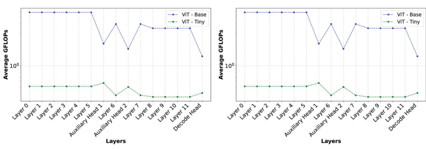
Figure 8.3 Layer-by-layer analysis considering GFLOPs and Throughput (FPS) for pruning heads placed at positions 6 and 8
