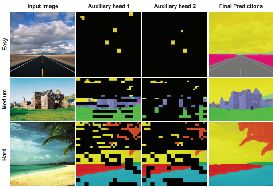
Figure 8.4 ViT-Base segmentation results with pruned tokens masked in black
