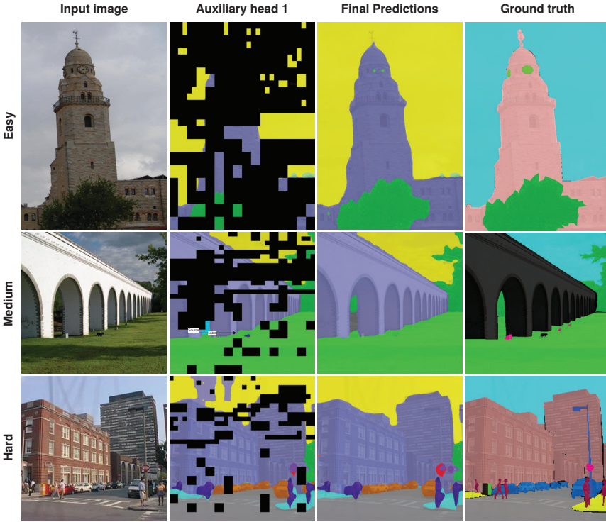
Figure 8.5 ViT-Tiny segmentation results with pruned tokens masked in black
