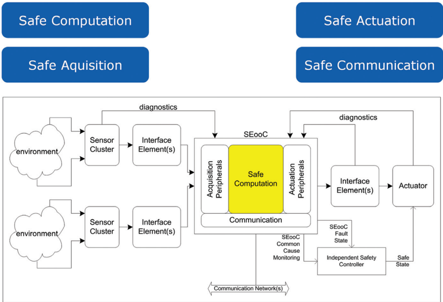
Figure 2.16 SEooC safety mechanisms.
