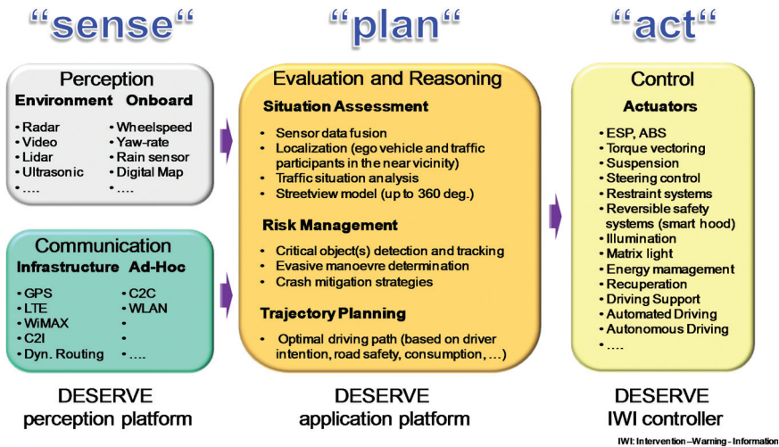
Figure 9.10 DESERVE platform.
