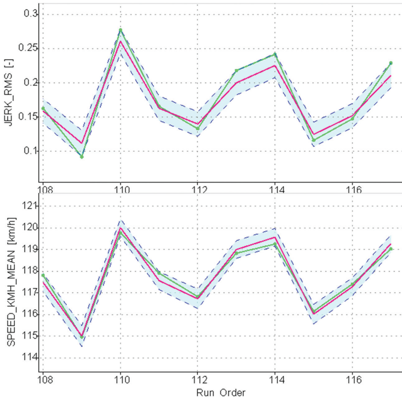
Figure 5.21 Verification plot to see how well the measured results from the verification run fit the model results.
