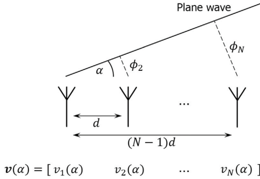
Figure 7.8 Uniform linear antenna array with spacing d and resulting steering vector \mathbf{v}(\alpha) .
