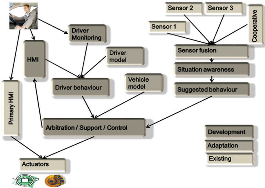
Figure 2.10 DESERVE platform architecture.
