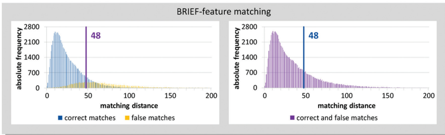
(c) Case study: BRIEF-feature matching
