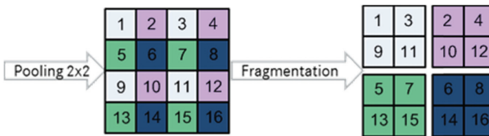
Figure 6.3 Example of a fragmentation after a 2 \times 2 pooling. The naïve approach would only produce the bright pixels, while an overlapping pooling produces all other possible pixels (purple, green, and blue). These pixels must be reordered to be able to correctly continue with the forward propagation of the neural network.
