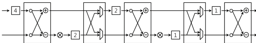
Figure 7.10 Radix-2 FFT implementation based on a multi-path delay commutator (MDC) pipeline.
