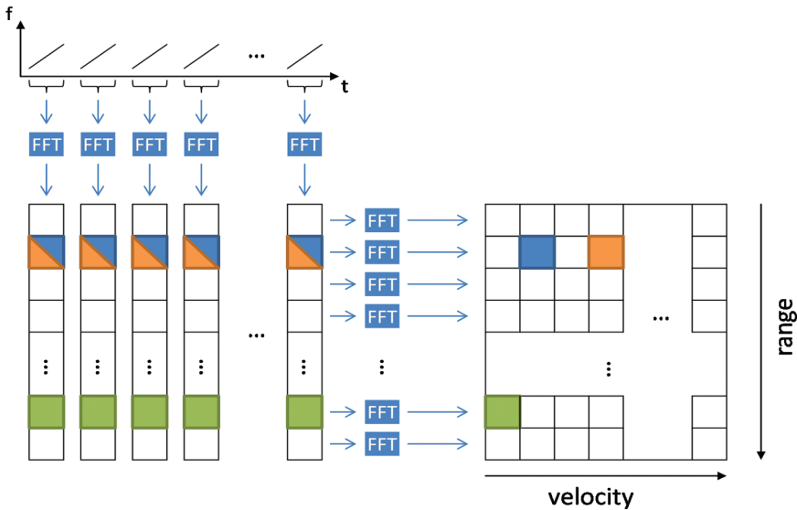
Figure 7.2 Chirp-sequence modulation.
