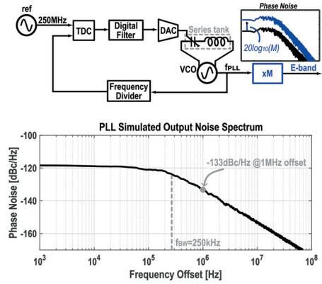
Fig. 14. Indirect LO synthesis approach through a DPLL (with series-resonance VCO) followed by a frequency multiplier, and simulated PLL spectrum.
