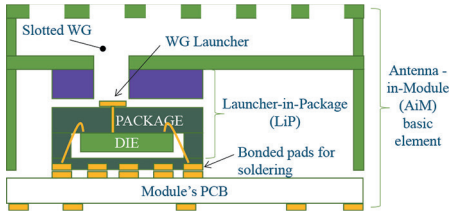
Fig. 2. First design of D-band AiM assembly.
