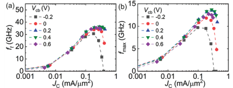
Fig. 10. (a) f_t and (b) f_{\text{max}} for a device with W_E : 5 \mu\text{m} and 55 nano-ridges ( L_E : 44 \mu\text{m} ) as functions of current density J_c . At V_{\text{ch}} = 0.4 V, extracted peak f_t is \sim 36 GHz and peak f_{\text{max}} is 13.7 GHz [24].
