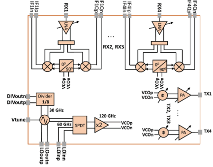
Fig. 6. The block diagram of the designed TRX for the in-cabin radar demonstrator developed in the BEYOND5 project.
