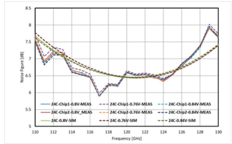
Fig. 7. TRX low-noise amplifier noise performance for the in-cabin radar demonstrator developed in the BEYOND5 project.
