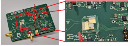
Fig. 5. 4 \times 4 MIMO TRX 22FDX chip for the in-cabin radar demonstrator developed in the BEYOND5 project.
