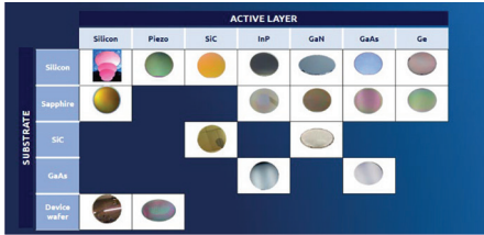
Fig. 2. Smart Cut technology combining an adapted active layer on a functional support substrate for a less dependent value chain.
