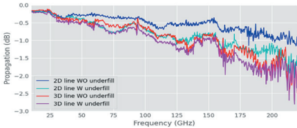
Fig. 2. Transmission line propagation in 2D and 3D contexts.
