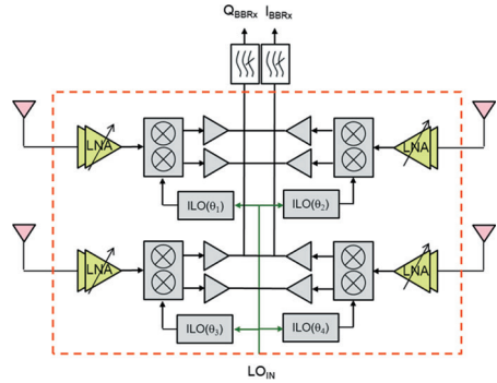
Fig. 7. Proposed receiver architecture.
