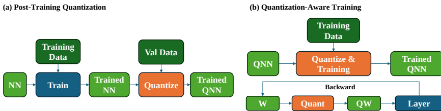
Figure 9.3 The workflow of the two main quantization methods: (a) Post-Training Quantization and (b) Quantization-Aware Training (including the straight throw estimator for the backpropagation)
