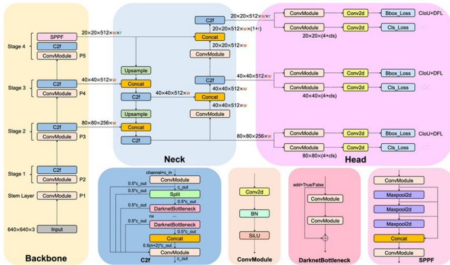
Figure 15.3 YOLOv8 architecture.
