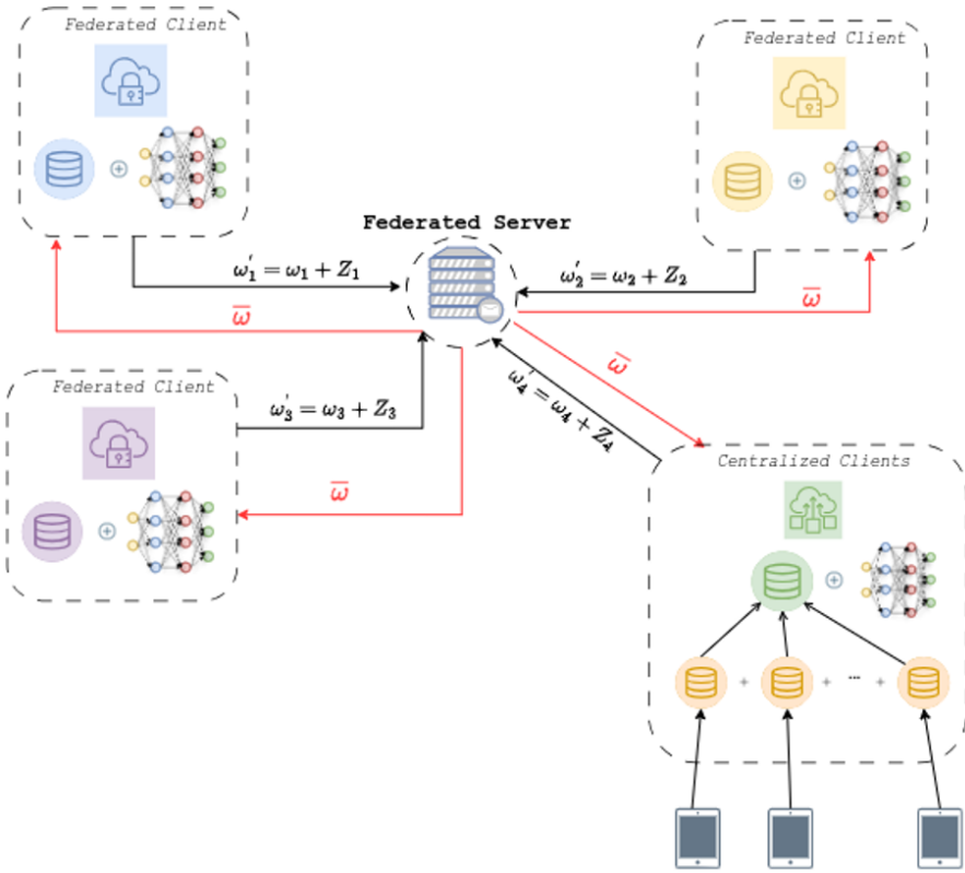
Figure 2.4 Implementation of the Vertical Hybridization in Flower
