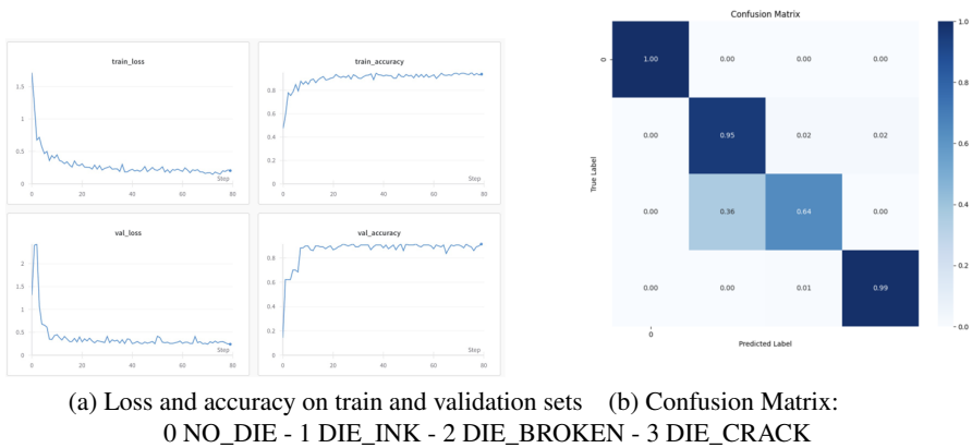
Figure 15.8 Metrics' trends during training and test result
