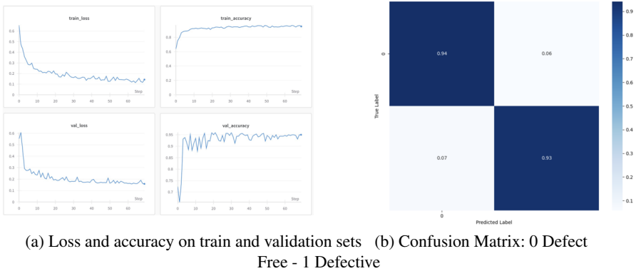
Figure 15.7 Metrics' trends during training and test result.
