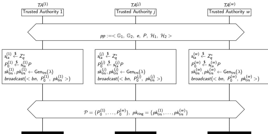
Figure 20.2 Network Bootstrapping.
