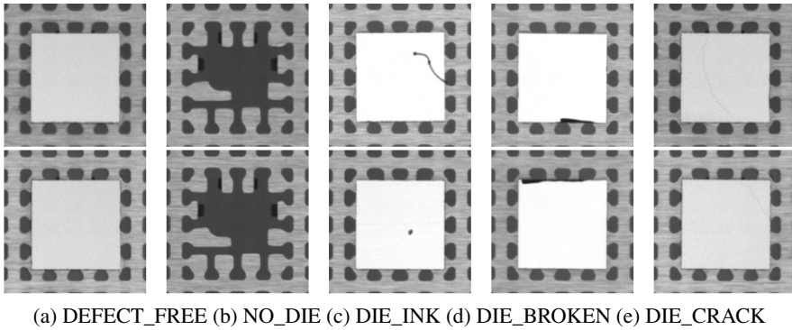
Figure 15.6 Defect-free chip and four common chip surface defects
